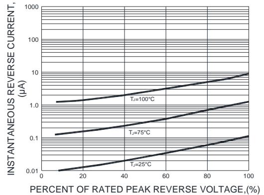
FIG.4-TYPICAL REVERSE CHARACTERISTICS
