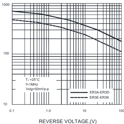
FIG.5-TYPICAL JUNCTION CAPACITANCE
